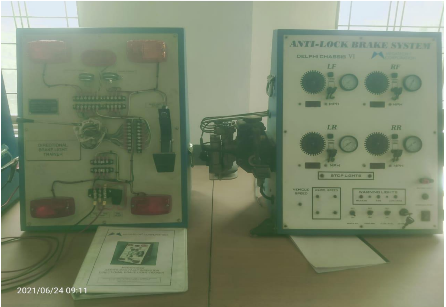
Directional Lights and Ani-Brake system
