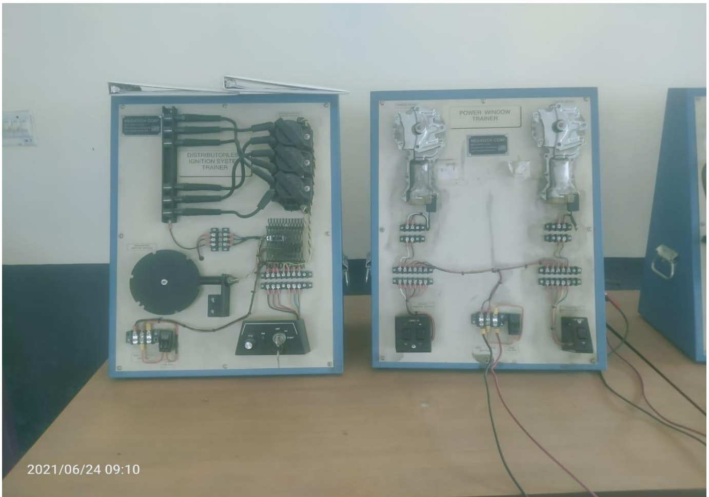
Directional Brake Light Trainer and Distributorless Ignition (DIS)
