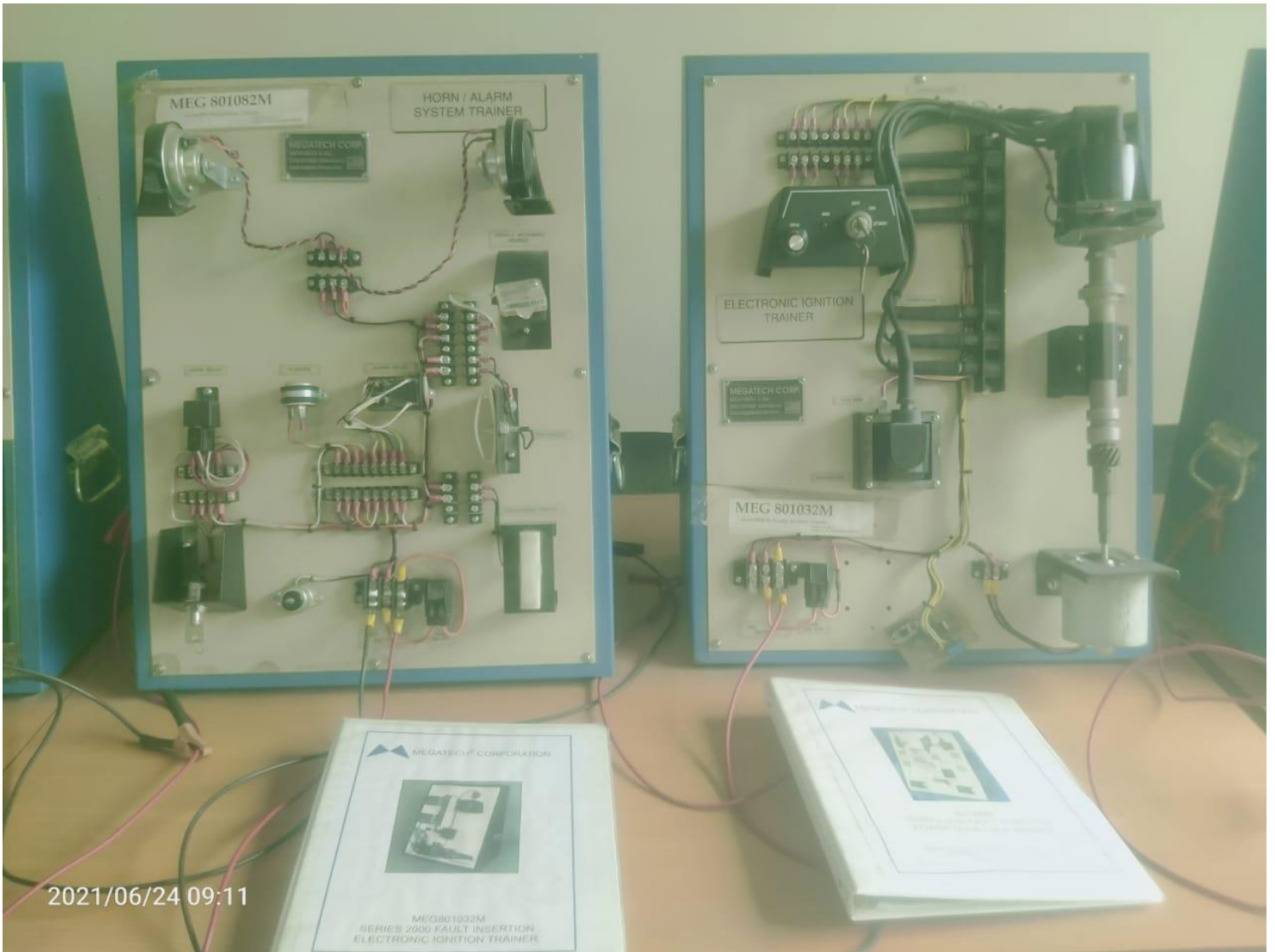
Horn and Alarm System Trainer and Electronic Ignition Trainer
