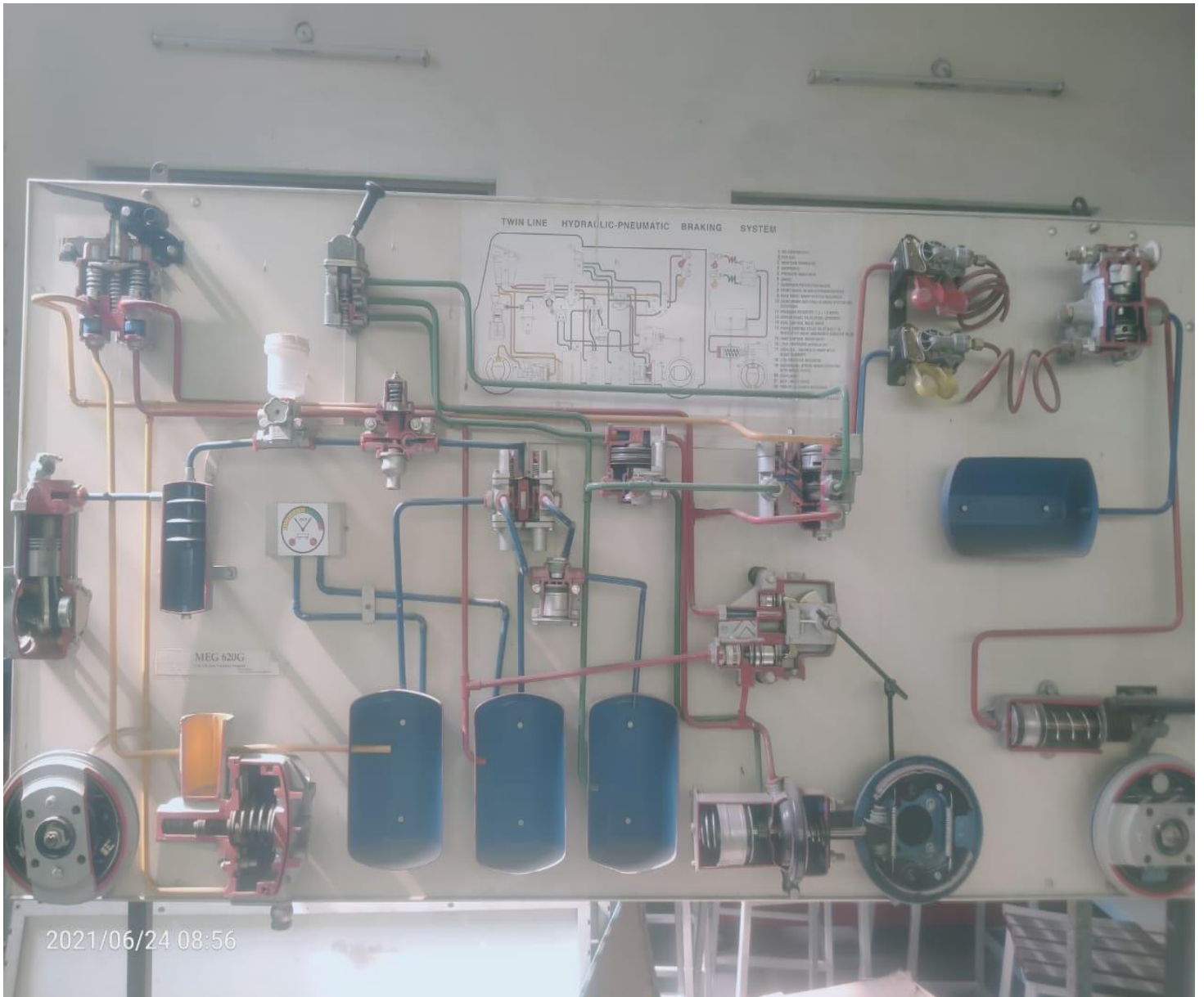
Hydraulic Pneumatic Braking System
