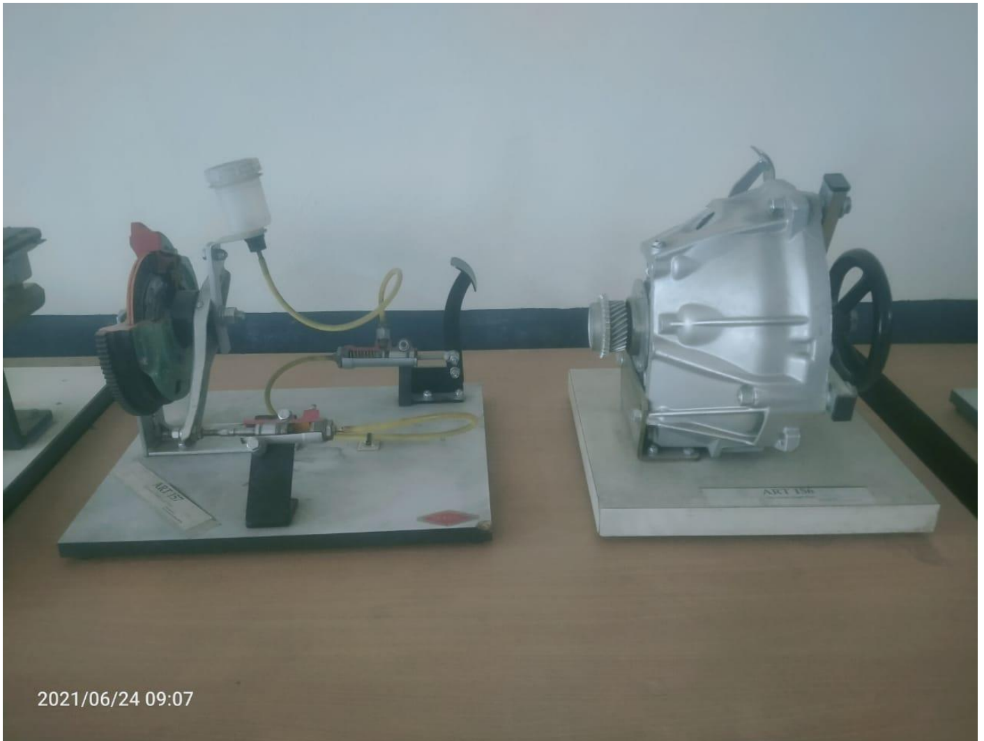
Hydraulic Clutch Single Plate and Dry Clutch Plate
