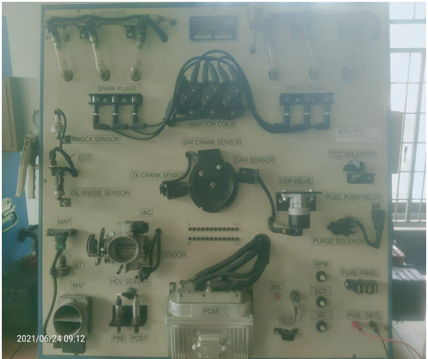
Multiport Fuel Injection
