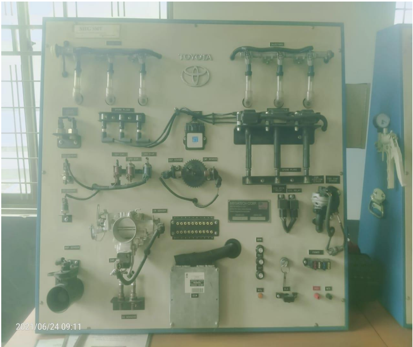
Multiport Fuel Injection Common Rail Diesel Trainer
